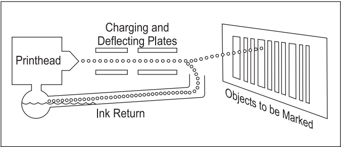
Figure 3. Ink Jet Printing
