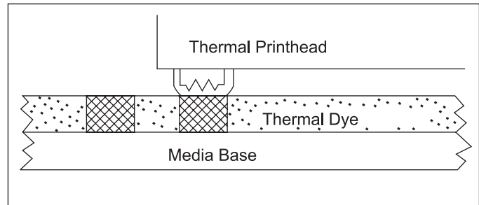
Figure 5. Direct Thermal Printing
