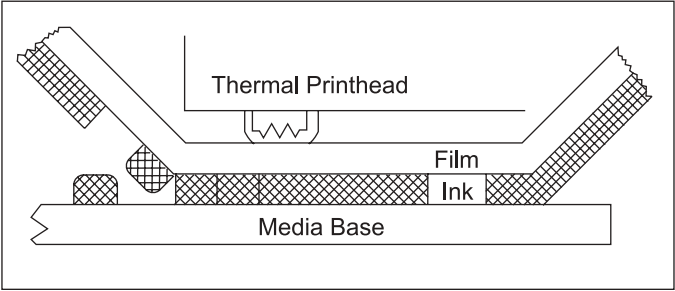
Figure 6. Thermal Transfer Printing
